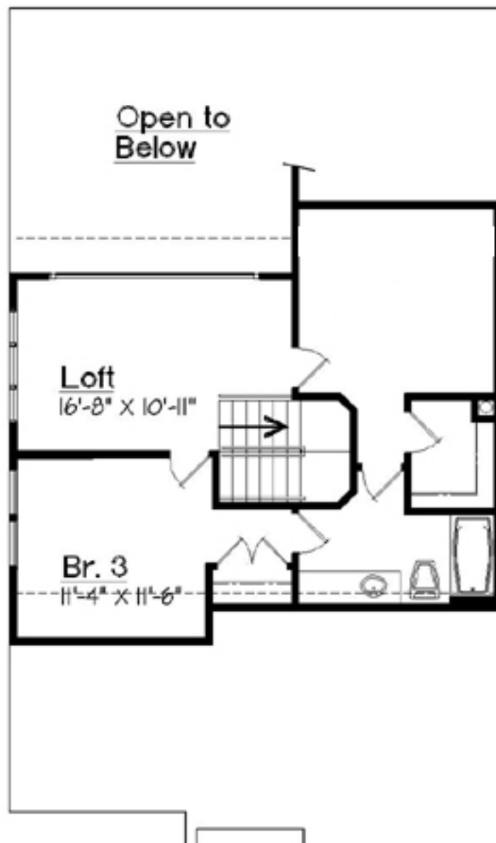
UNIT C - SECOND FLOOR
