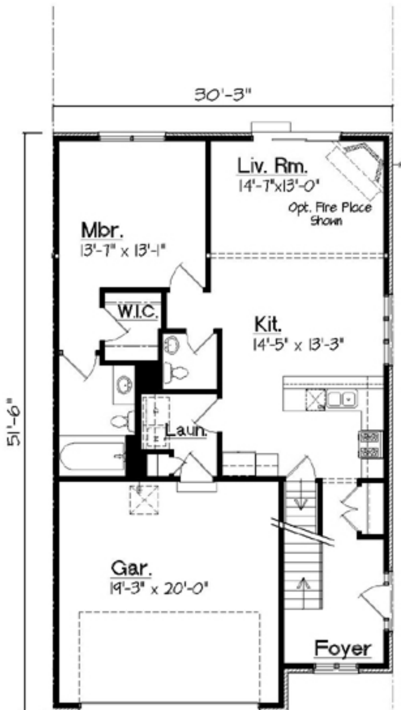
UNIT D - END UNIT FIRST FLOOR
